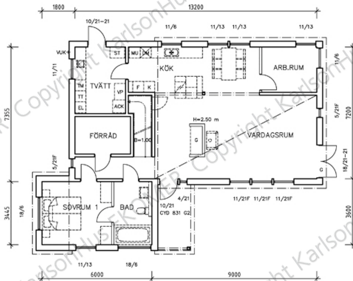
BOTTENPLAN BOA 116.4 m 2
